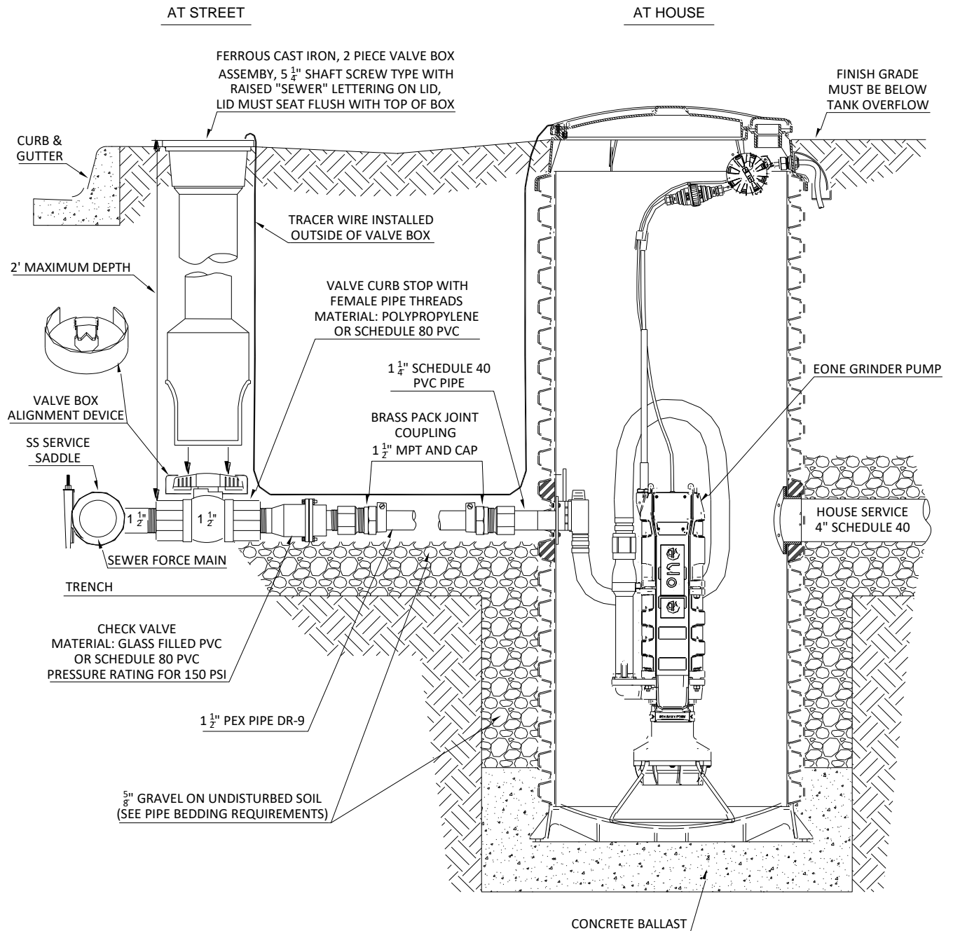
Installation Detail
