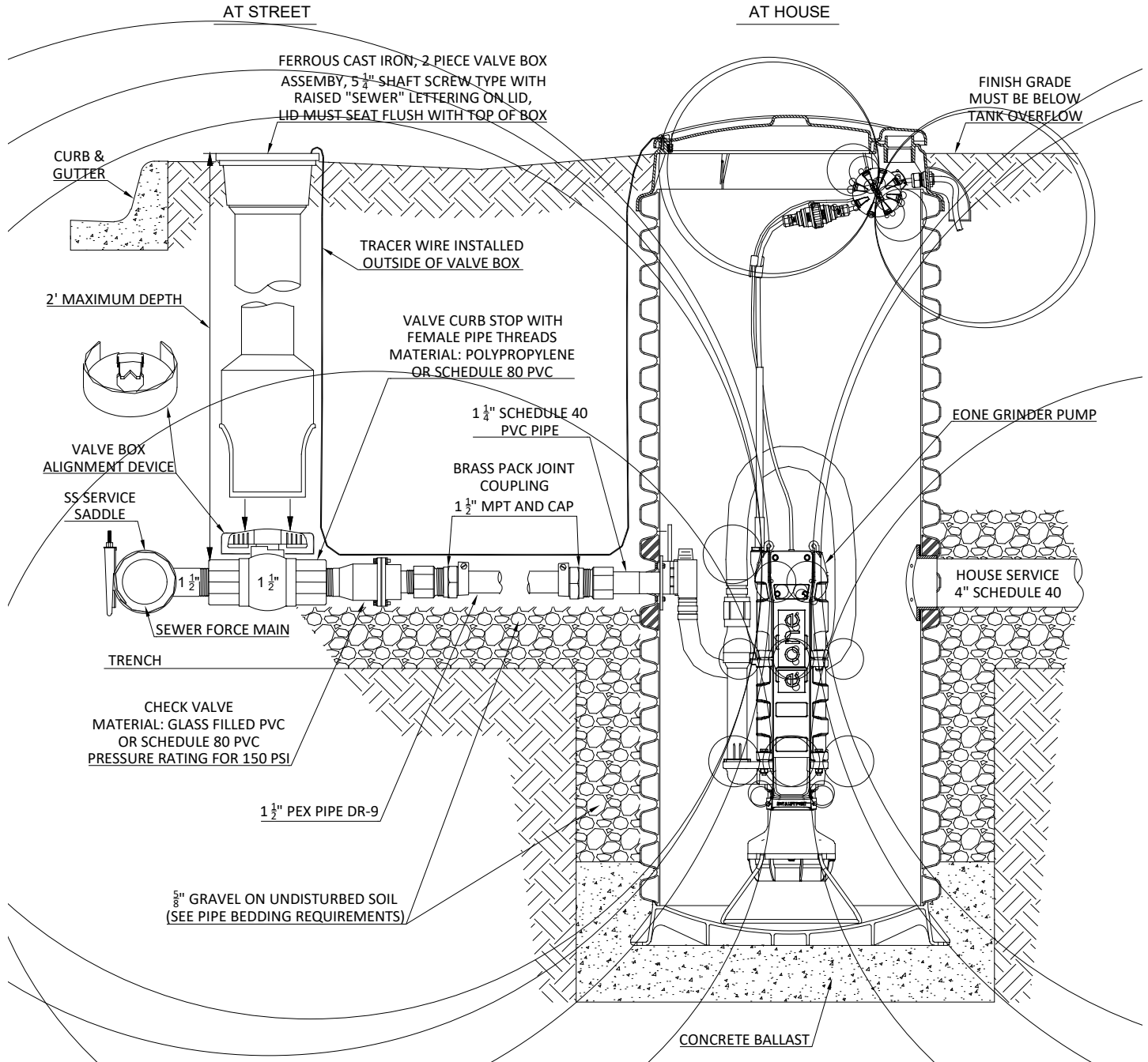
Installation Detail
