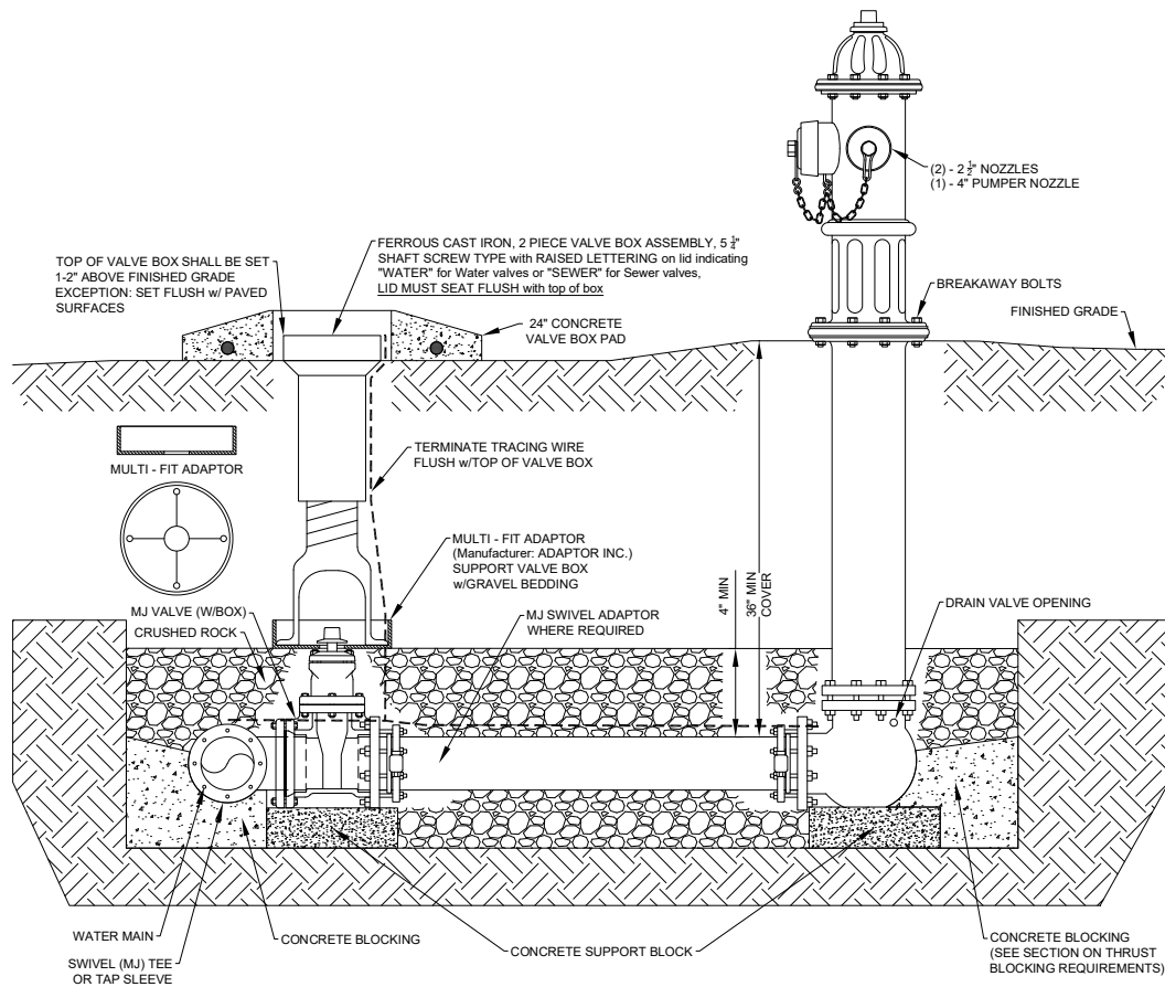
TYPICAL - FIRE HYDRANT ASSEMBLY NTS
