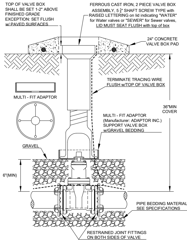
VALVE INSTALLATION DETAIL
